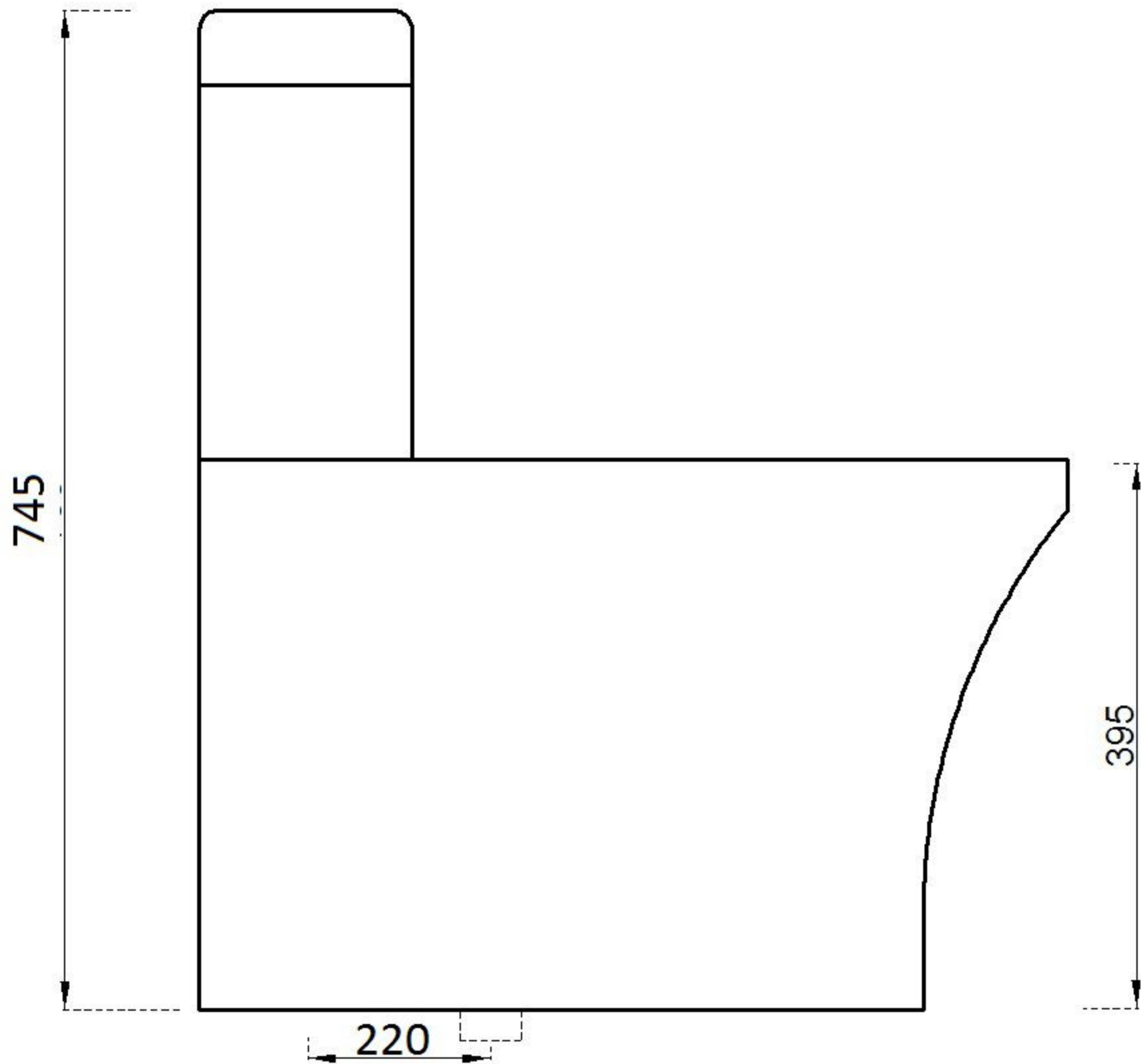
FRONT VIEW
