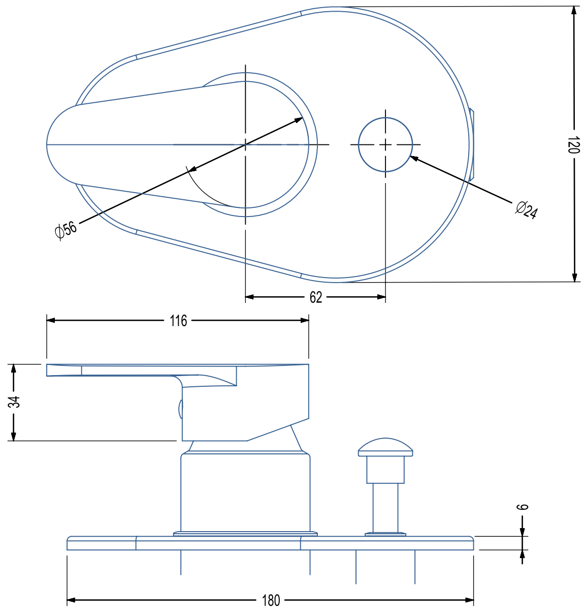
EXPOSED PARTS OF S/L CONCEALED DIVERTER HIGH FLOW - FVN112
