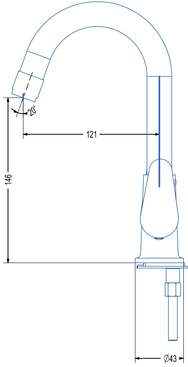
Sink Mixer With Swinging Spout Table Mounted - FRV066
