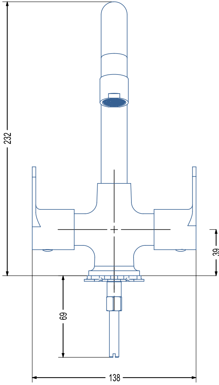
Sink Mixer With Swinging Spout Table Mounted - FRV066
