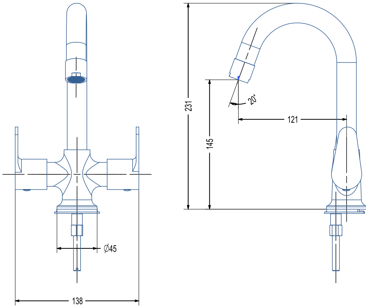
Center Hole Basin Mixer - FVN051
