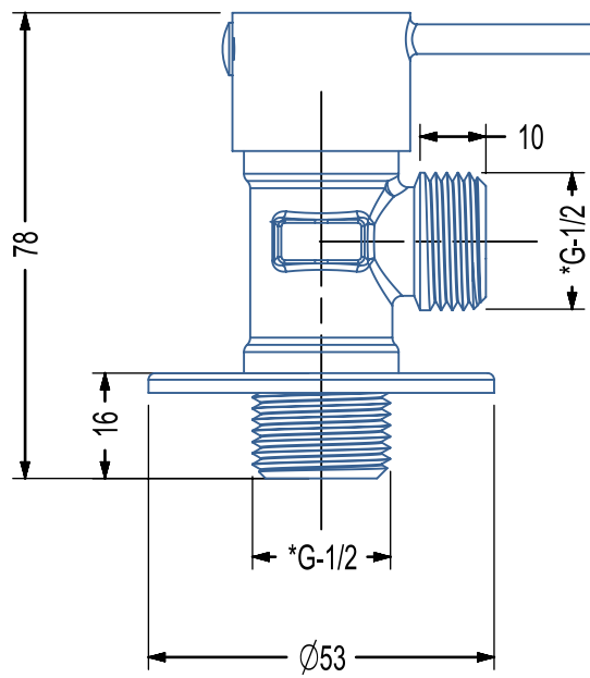
ANGULAR STOP COCK ORION CCN324 / CCN324F
